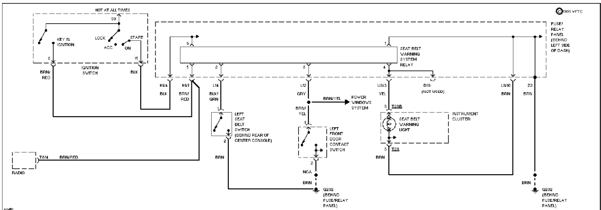
Warning System Circuits
