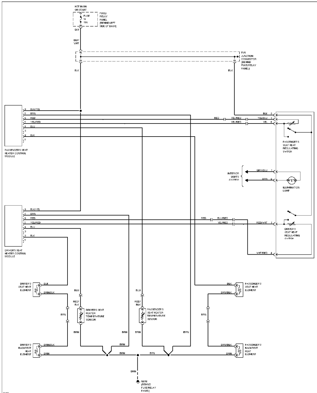
Heated Seats Circuit
